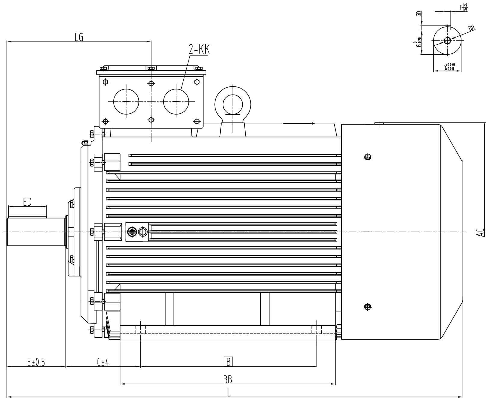
OUTLINE DIMENSIONS FOOT MOUNTED MOTOR
