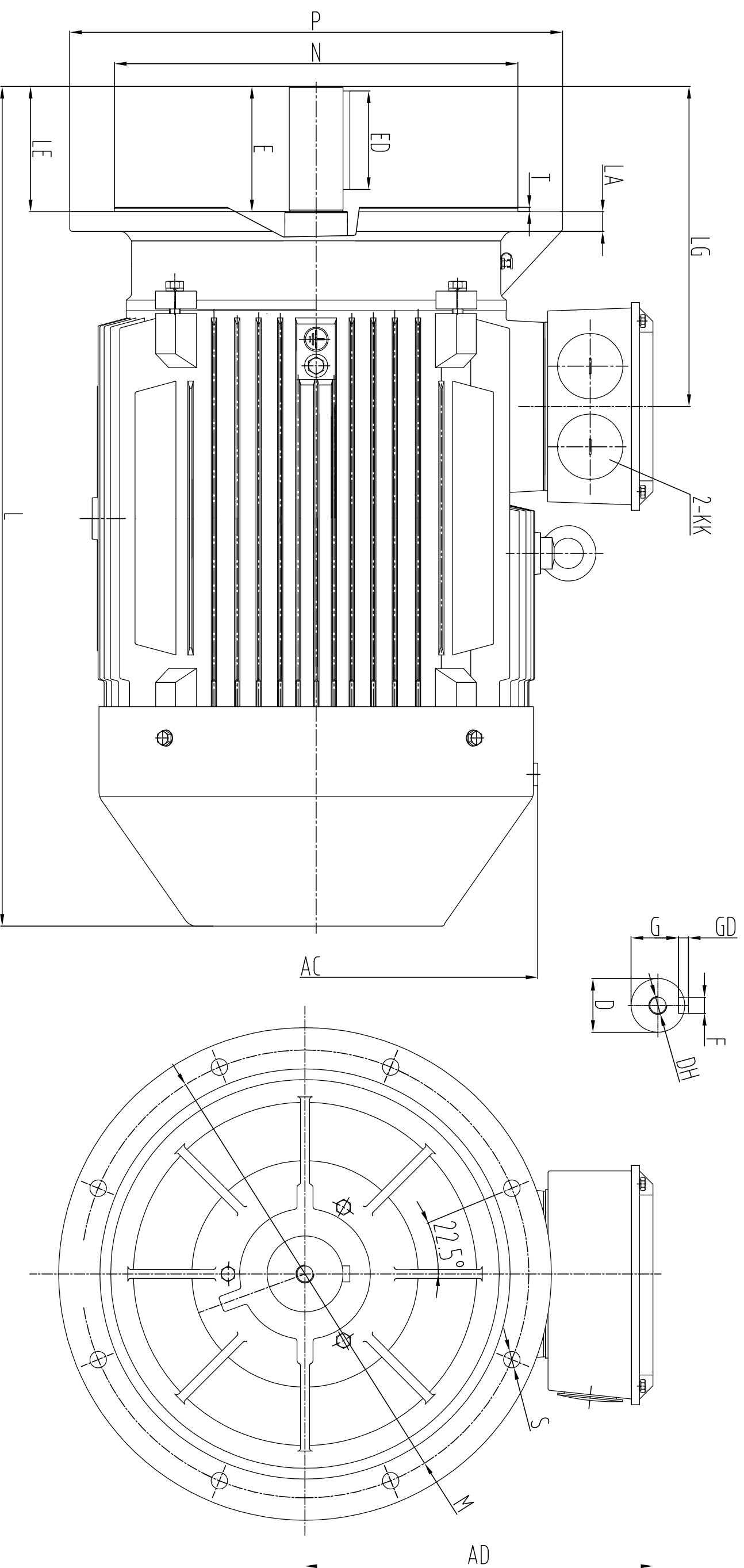
OUTLINE DIMENSIONS FLANGE MOUNTED MOTOR
