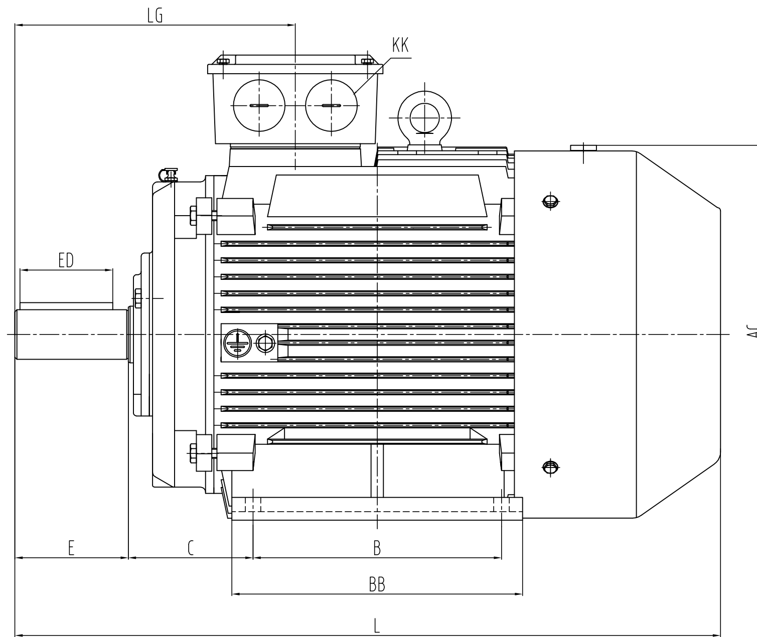
OUTLINE DIMENSIONS FOOT MOUNTED MOTOR
