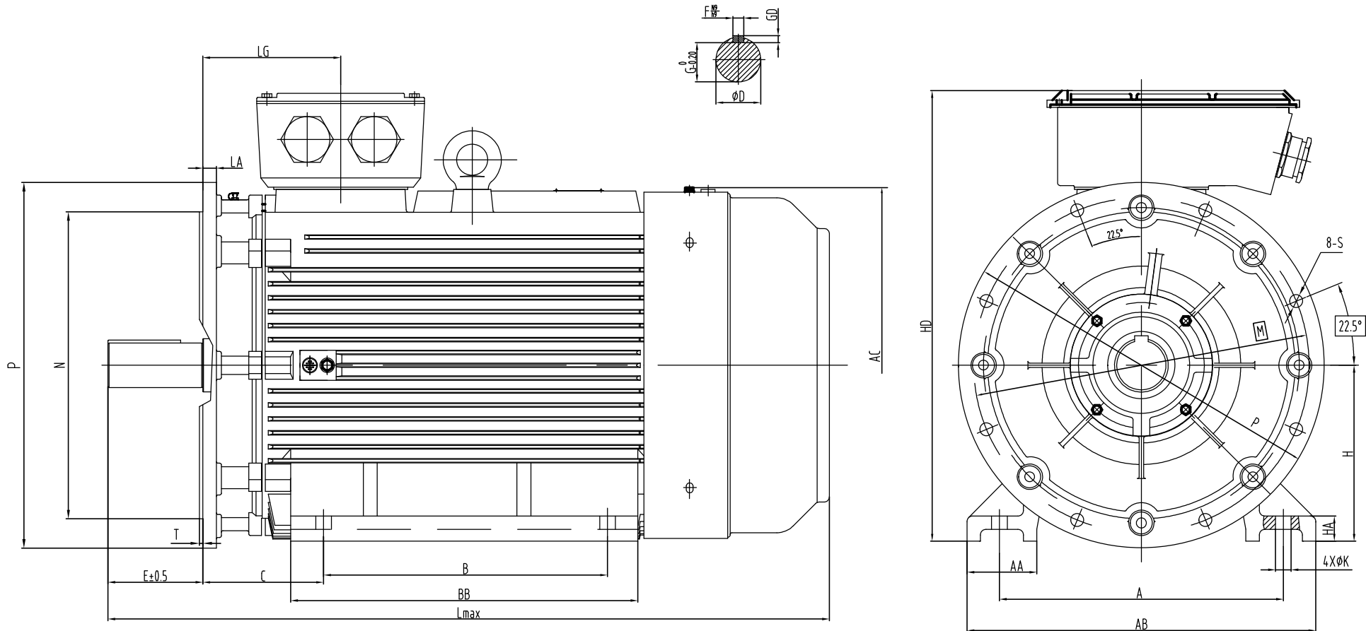
OUTLINE DIMENSIONS FOOT/FLANGE MOUNTED MOTOR
