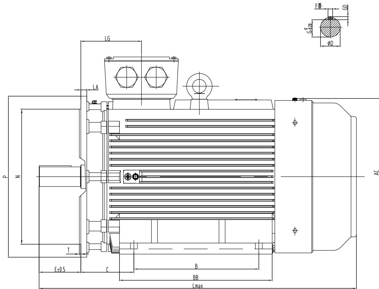
OUTLINE DIMENSIONS FOOT/FLANGE MOUNTED MOTOR
