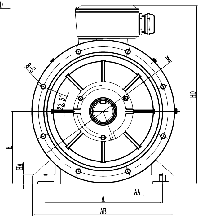
OUTLINE DIMENSIONS FOOT/FLANGE MOUNTED MOTOR
