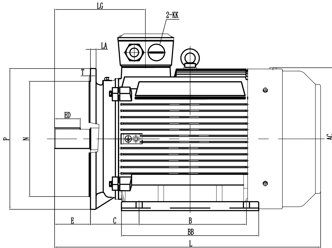
OUTLINE DIMENSIONS FOOT/FLANGE MOUNTED MOTOR
