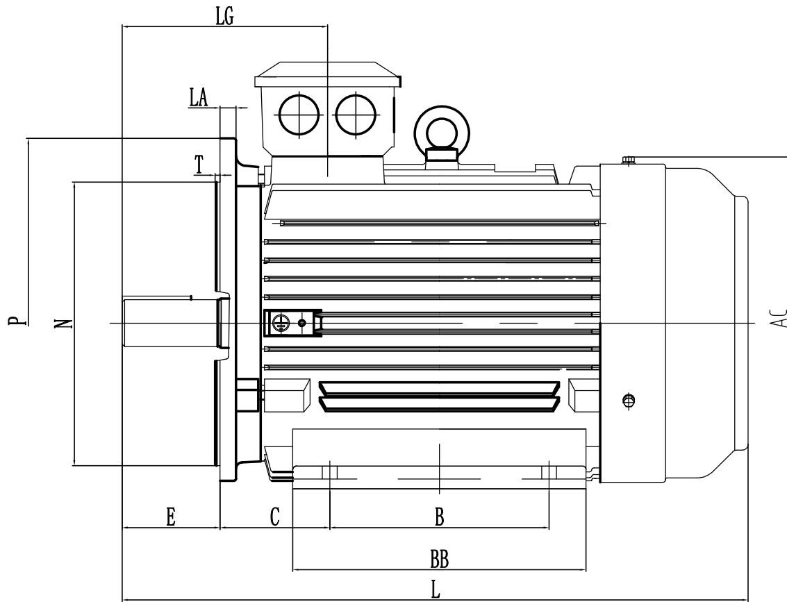
OUTLINE DIMENSIONS FOOT/FLANGE MOUNTED MOTOR
