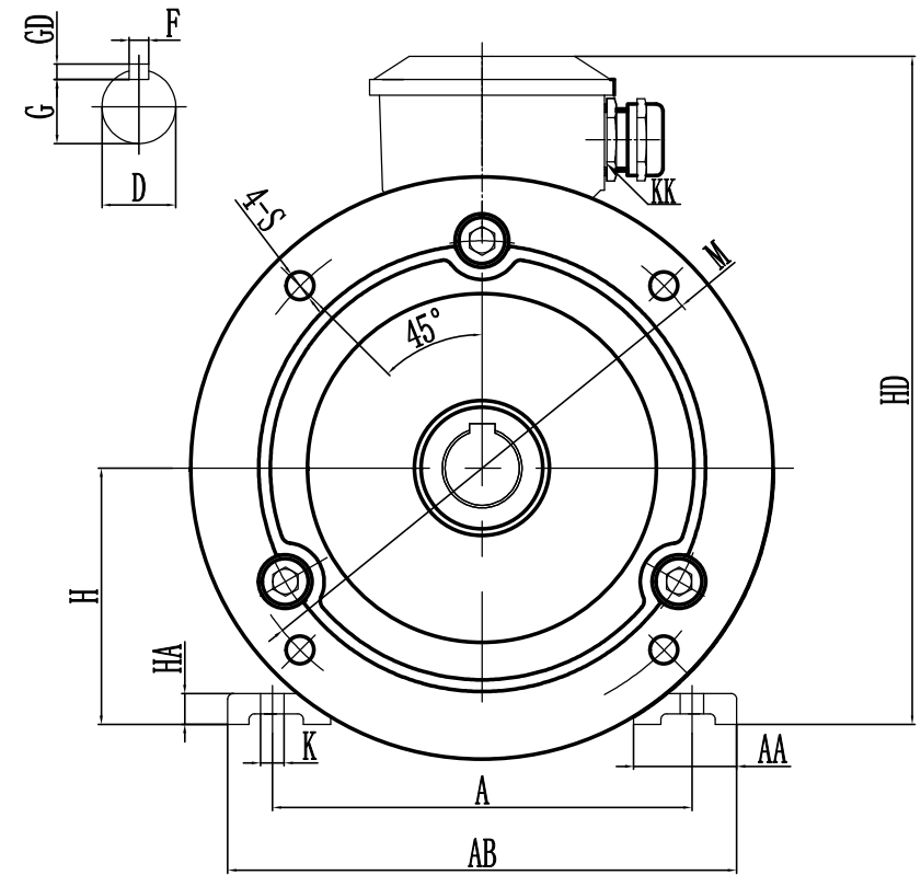
OUTLINE DIMENSIONS FOOT/FLANGE MOUNTED MOTOR
